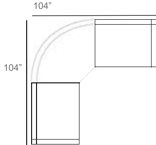
1 - Left 1 - Corner 1 - Right Patio Furniture Cover Size: 128" x 128" Sectional Cover 3008-0006
